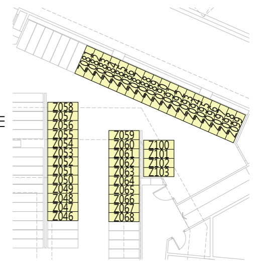
5 PART PLAN OF BICYCLE PARKING SPACE 單車停車位部份平面圖
