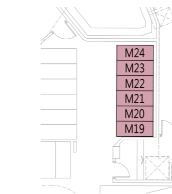
1 PART PLAN OF RESIDENTIAL MOTOR CYCLE PARKING SPACE 住宅電單車停車位部份平面圖
