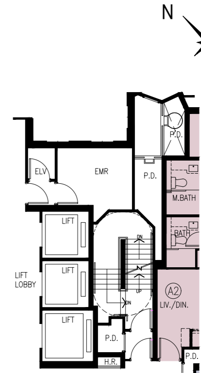
PART PLAN OF STAIRCASE AT 3/F 3樓樓梯部分平面圖
